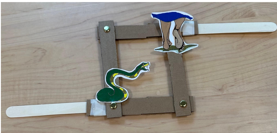
Parallel Motion Device With 4-Bar Linkage
