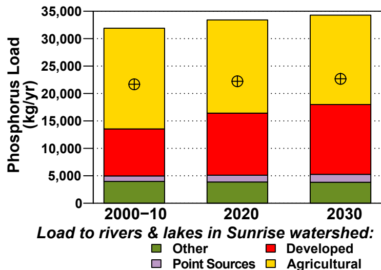
Figure 2. Phosphorus loads from selected land use categories to rivers and lakes in the Sunrise River watershed (bars) and loads exported from the Sunrise to the St. Croix River (symbol), for baseline (2000-10) and projected (2020-2030) conditions.
