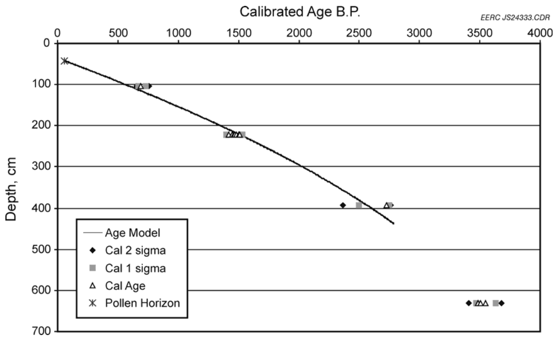
Figure 7. Age model.
