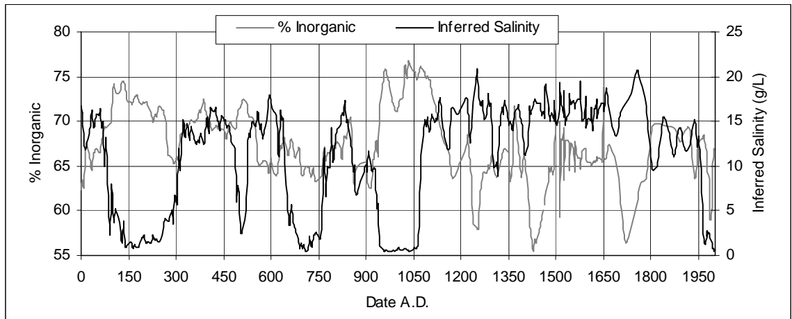
Figure 9: Loss on ignition and inferred salinity
