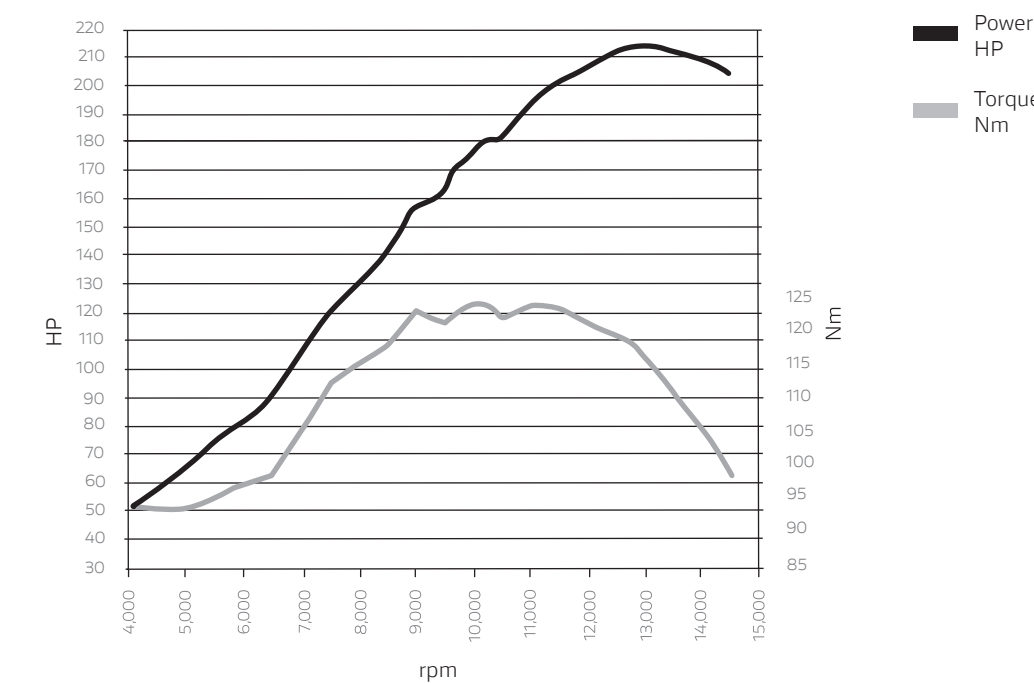
Power and torque
