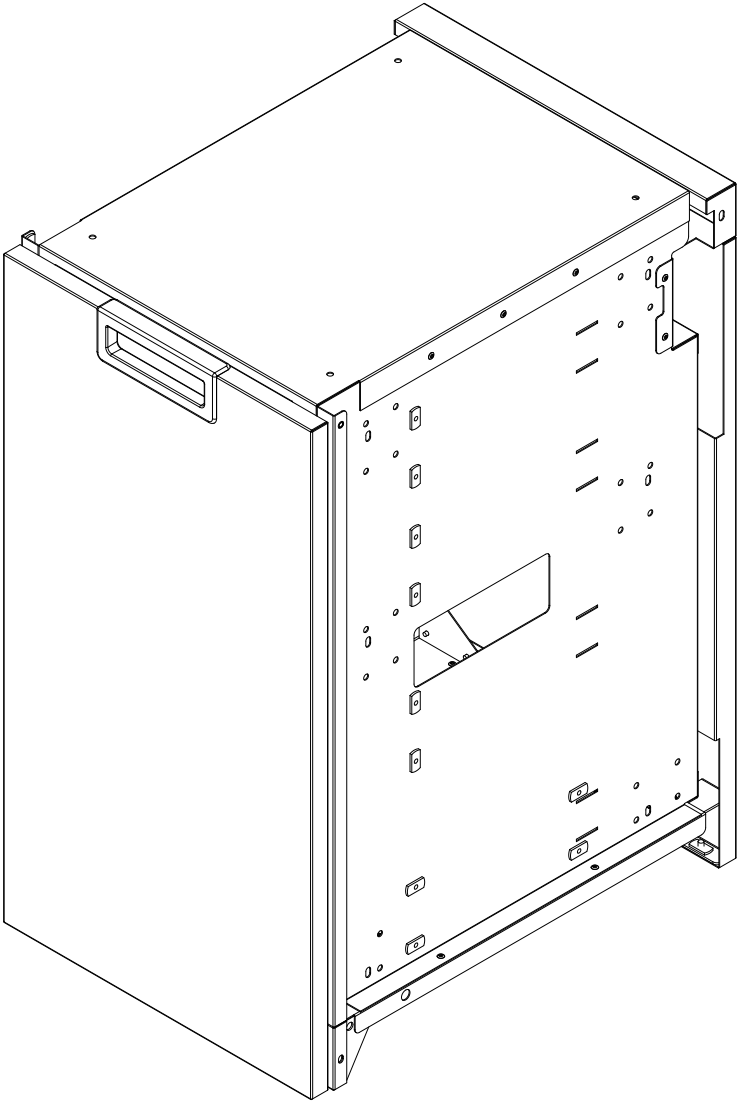
Door shown with righthand mounting option. Door hardware can be switched for lefthand mount.
