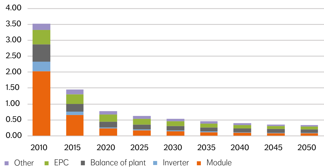
Figure 2: Global capex cost forecast utility-scale PV solar ($/W)
