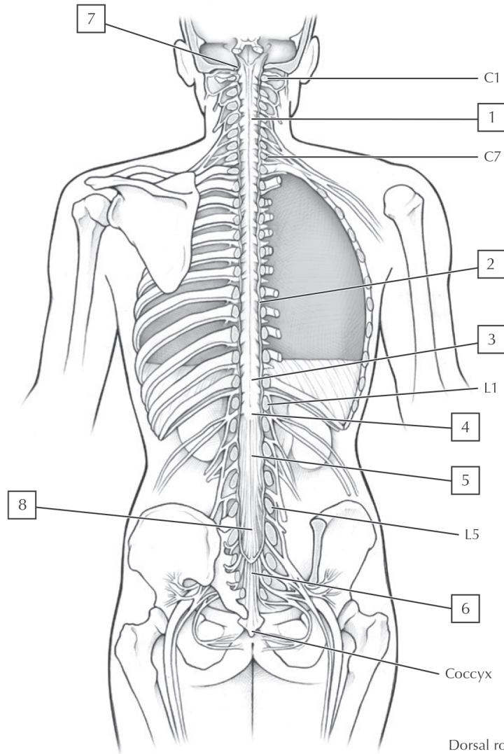
A. Spinal cord gross anatomy in situ
