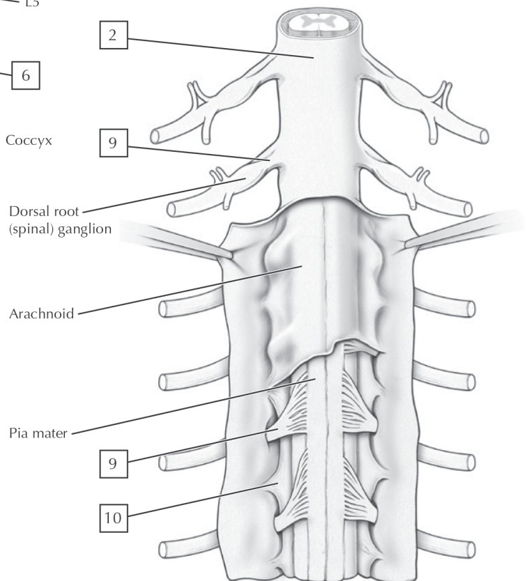
B. Meninges and spinal roots
